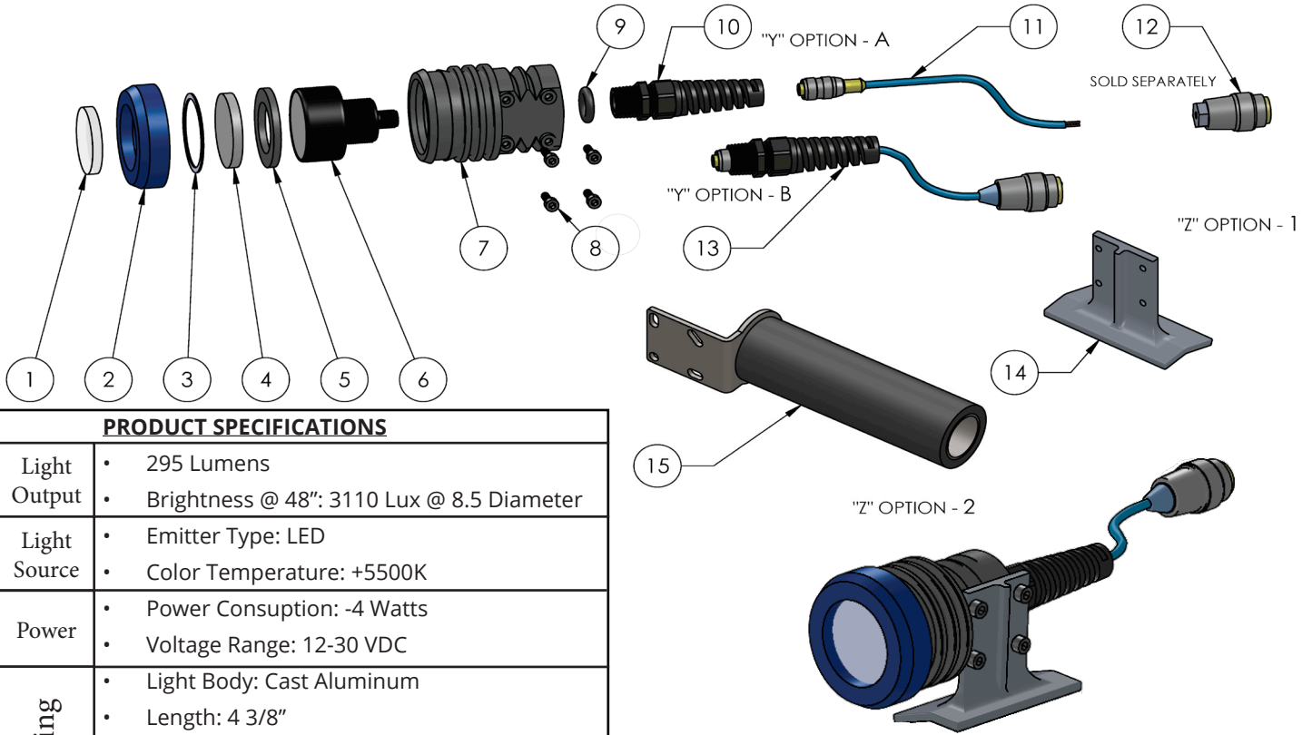
SAMPLE CONFIGURATION: 630531B1 HOSE MOUNT, POWER CORD WITH CONNECTOR
